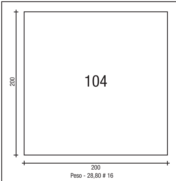
COLUNA 200 X 200 # 16
