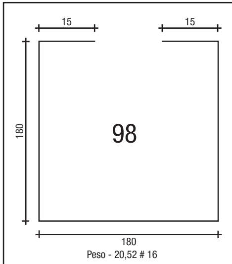
COLUNA 180 X 180 # 16
