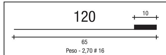
TAMPA G # 16
