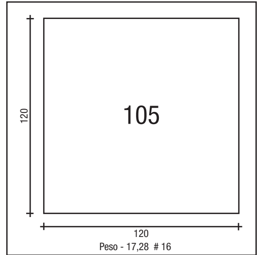
COLUNA 120 X 120 # 16
