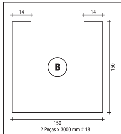
COLUNA LATERAL
