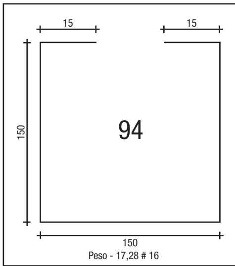
COLUNA 150 X 150 # 16
