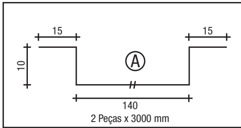
TAMPA COLUNA LATERAL
