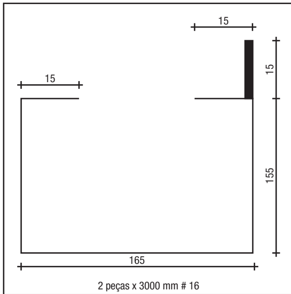
COLUNA LATERAL
