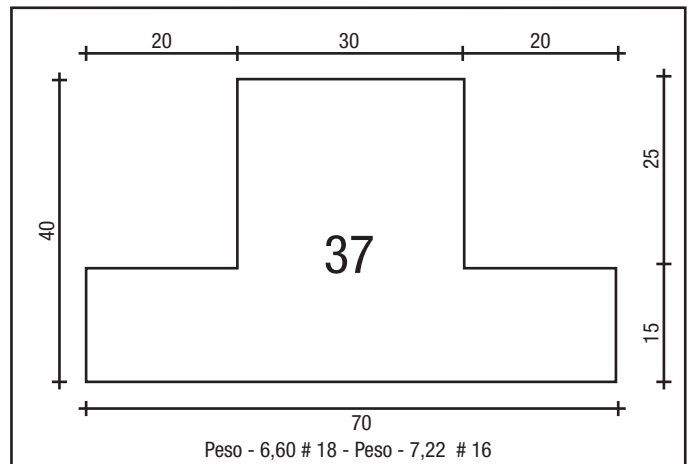
TEE MAX BICO 15
