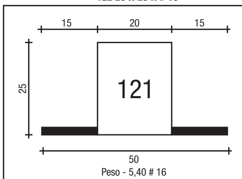
TEE 20 X 25 X # 16
