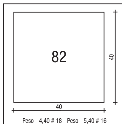
COLUNA 40 X 40
