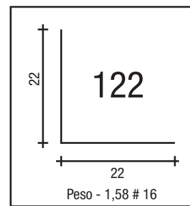
TRAVA 22 X 22 X # 16
