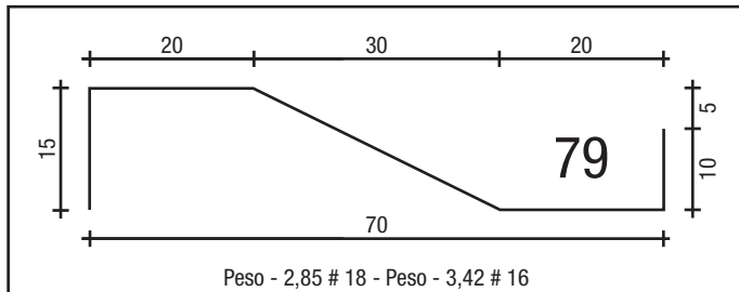
COLUNA 50 X 25
