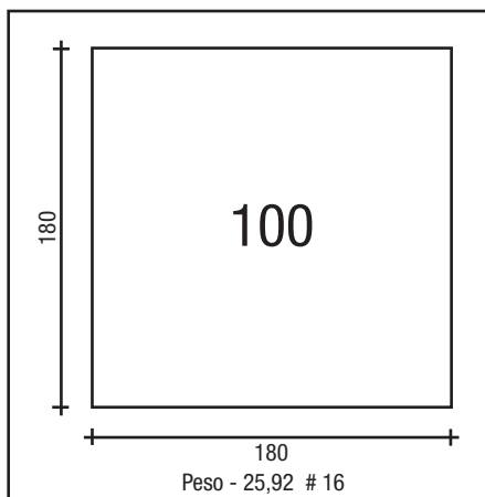
COLUNA 180 X 180 # 16
