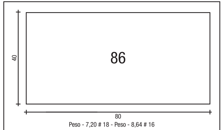
COLUNA 80 X 40
