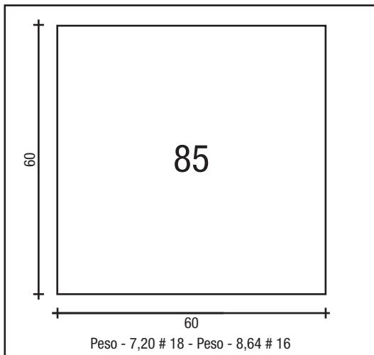
COLUNA 60 X 60
