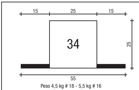
TEE 25 X 25
