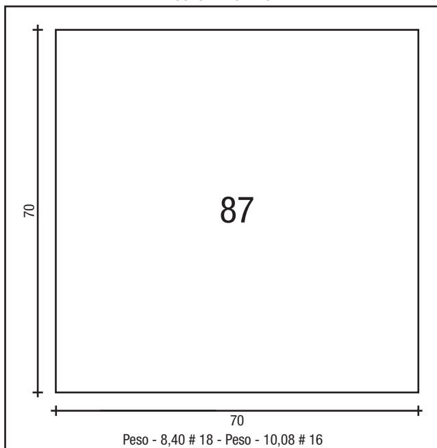
COLUNA 70 X 70
