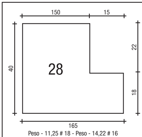
ALMOFADA COM GRADE 150 X 40
