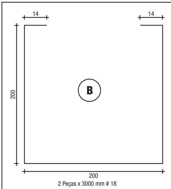
COLUNA LATERAL
