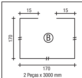
COLUNA LATERAL
